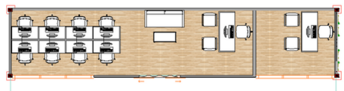
40 ft office unit with a separate exclusive office unit.
