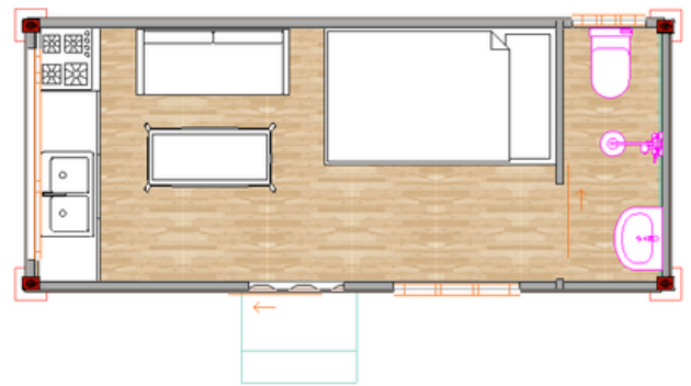
20 ft home with an open layout
