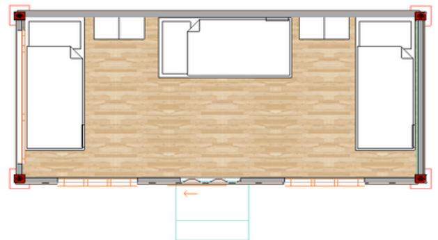
20 ft accommodation unit which can host upto 6 people.
